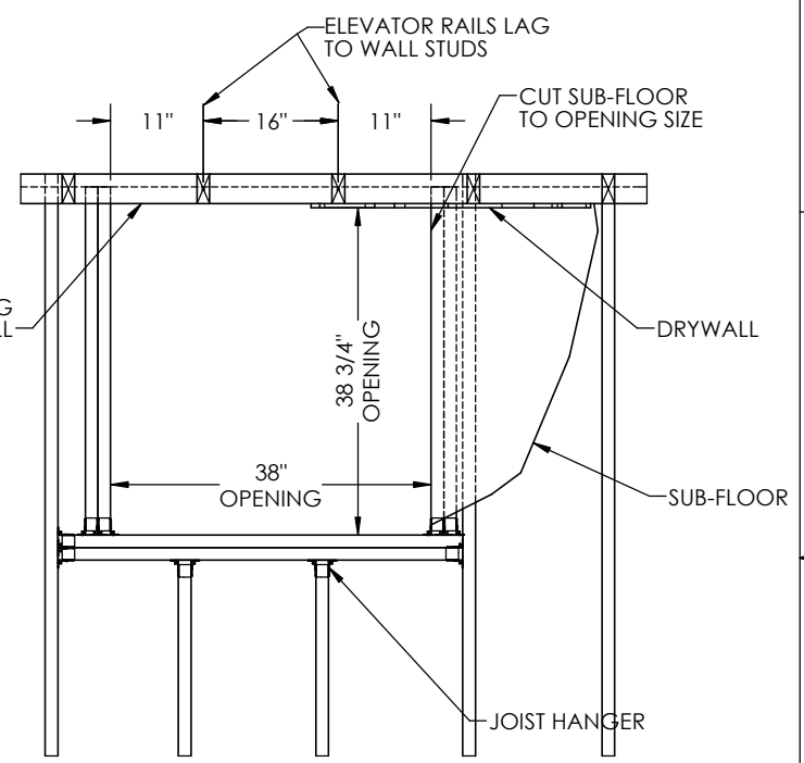
PLAN VIEW SCALE 1 : 16
