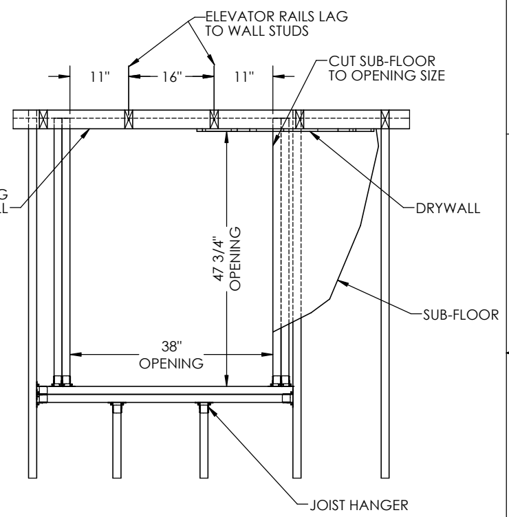
PLAN VIEW SCALE 1 : 16
