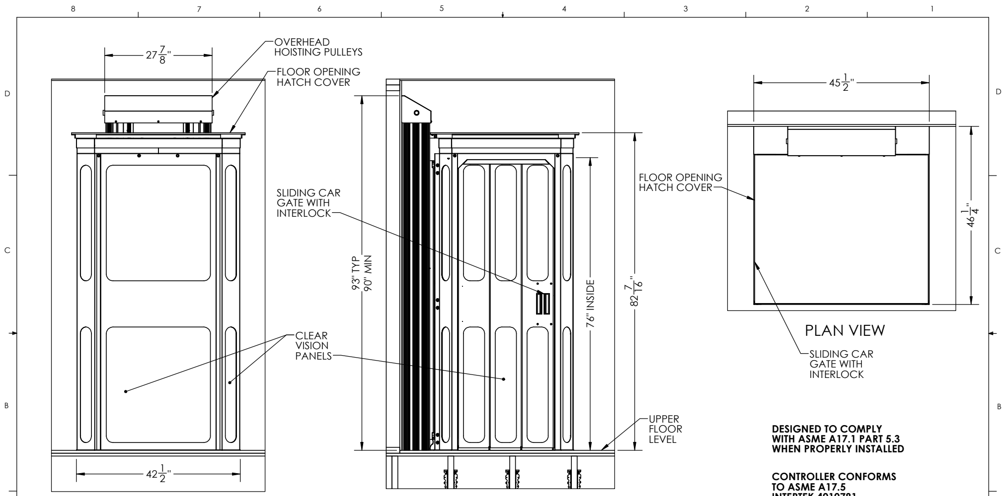
FRONT VIEW
